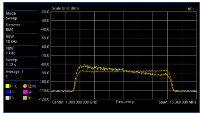
Figure 4. PIM detection
