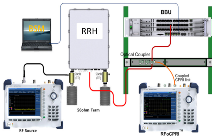
Figure 5. Calibration procedure
